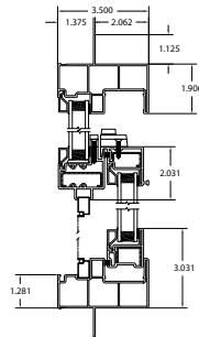
Horizontal Slider
