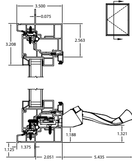
Casement Vertical
